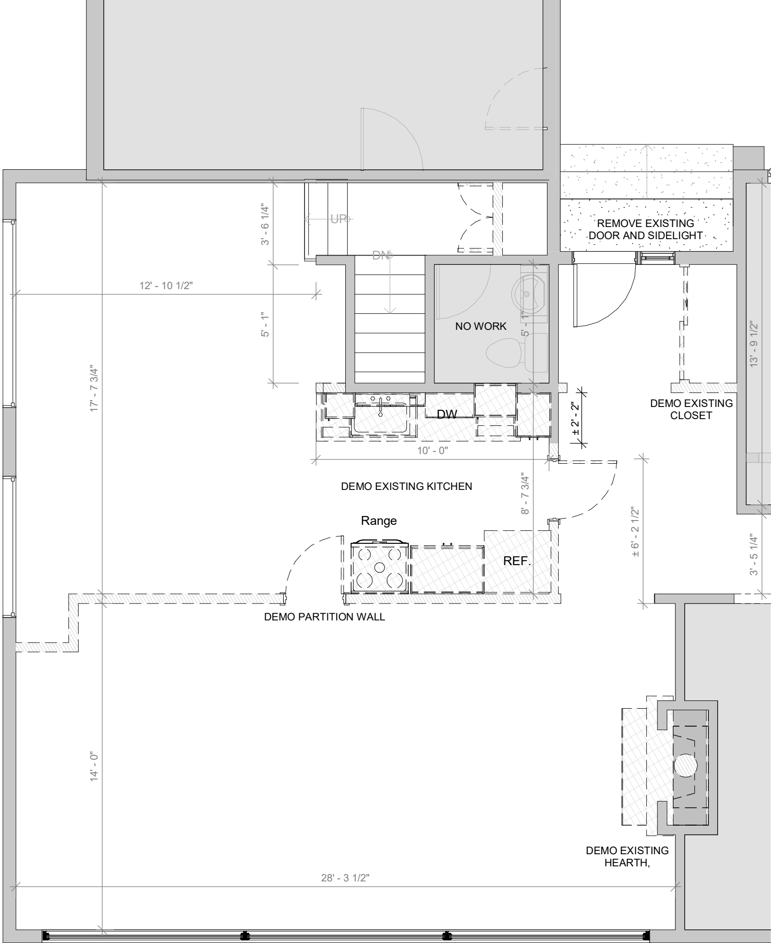
BEFORE - 1st FLOOR PLAN
