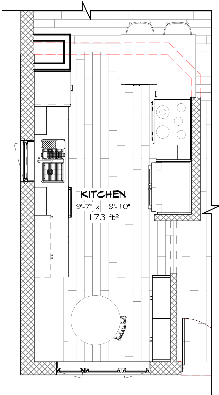
KITCHEN FLOOR PLAN
