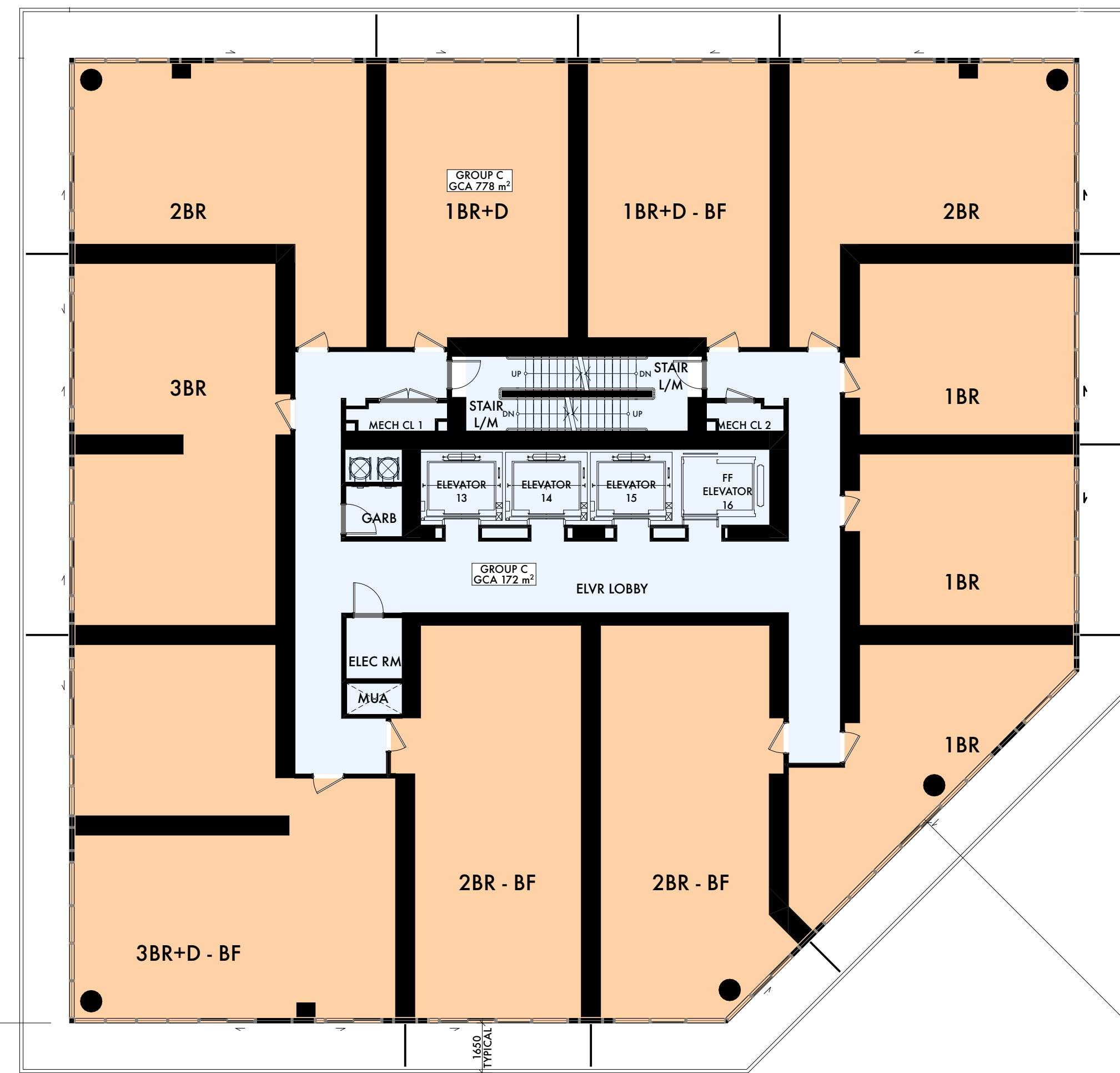
TOWER G, TYP. LEVELS 56 - 71
