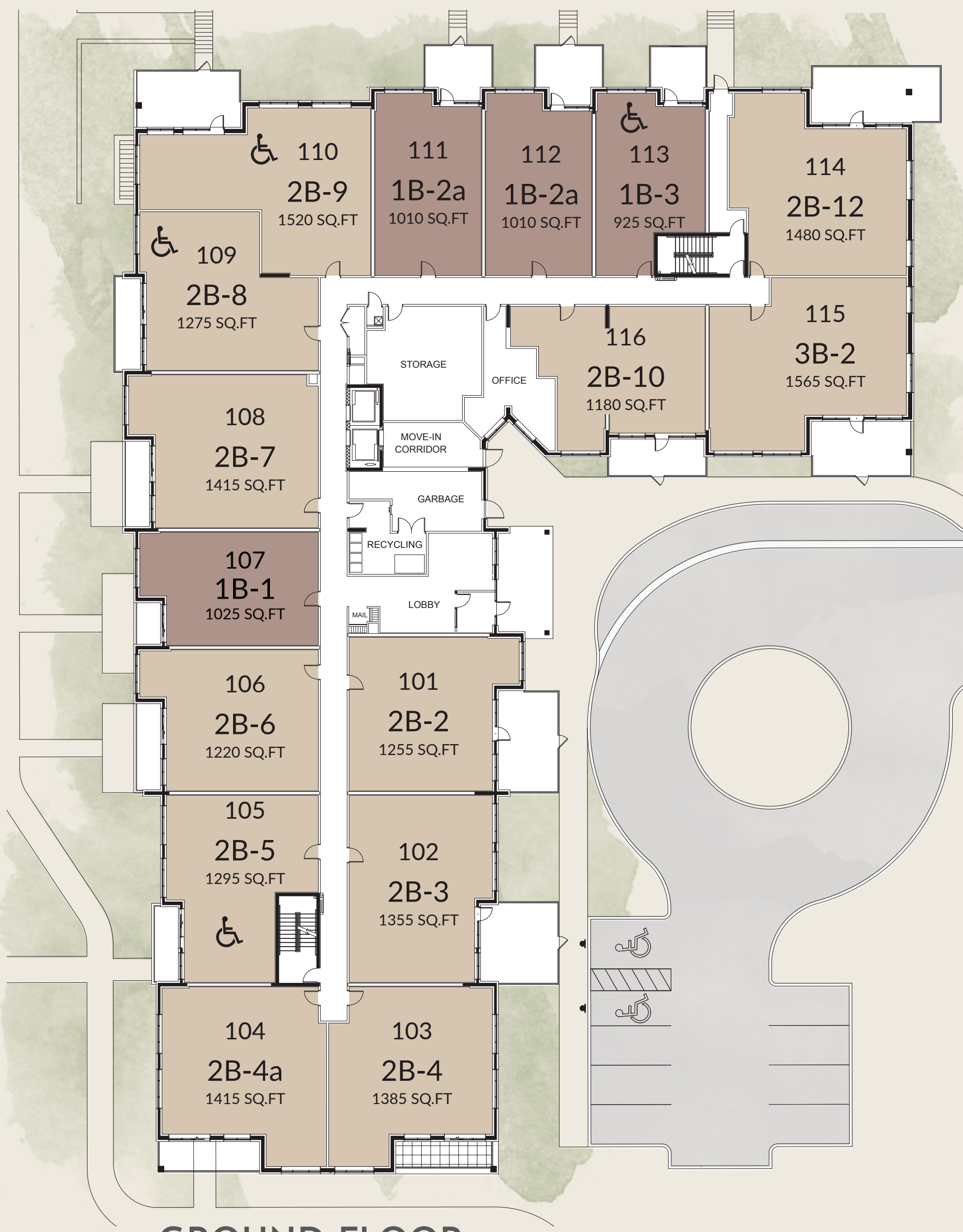
GROUND FLOOR
